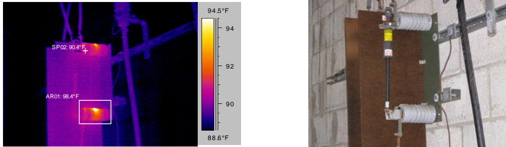
Figure-8a & 8b: A temperature rise of 8 F-degrees is observed on active corona on a 13kV stand-off bushing for a disconnect switch.
