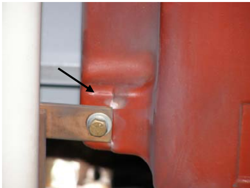
Figure-2: A sharp edge on a piece of copper bus provides an excellent spot for corona activity.
