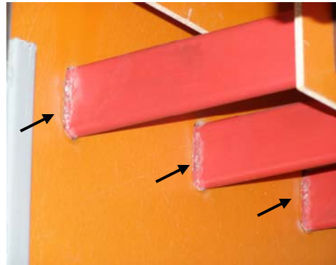
Figure-3: Corona deposits resulting from small air gap spaces between insulation board and 13kV bus bars.
