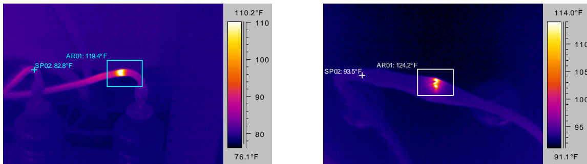
Figure 9a & 9b: Delta temperatures of over 30F-degrees are seen on conductor cables that having tracking problems.
