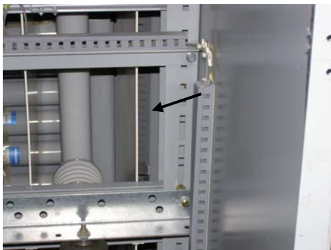
Figure 10a: Ultrasound was used to find tracking on blind side of insulation board (see arrow).
