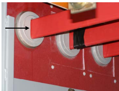
Figure 10b: Ultrasound was used to find corona on ceramic collars surrounding 13kV bus, no visible signs of corona are present.
