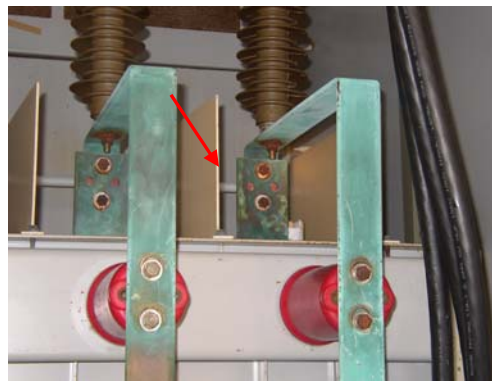
Figure-7: Unusual weathering pattern on 13kV copper bus under attack by corona produced nitric acid.
